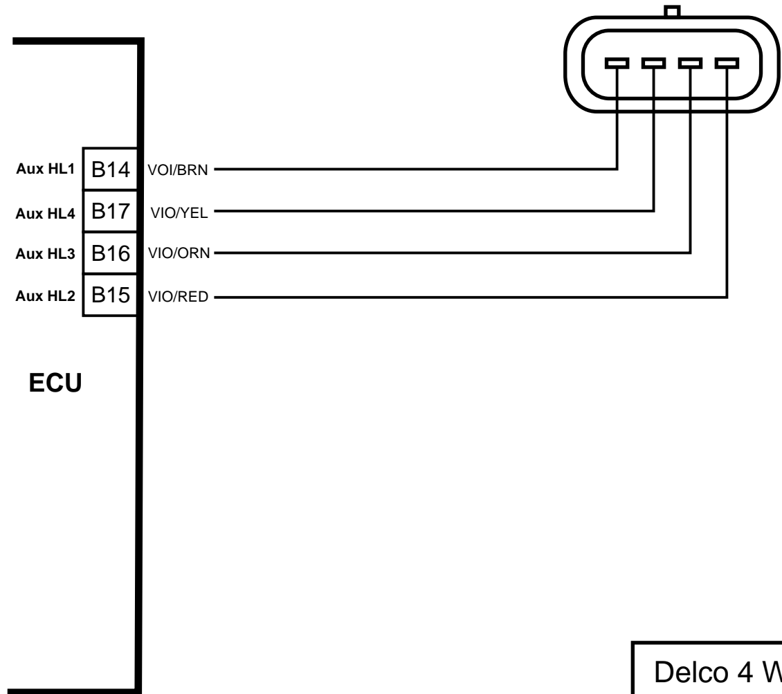
Stepper Motor Connector Male Pin View
